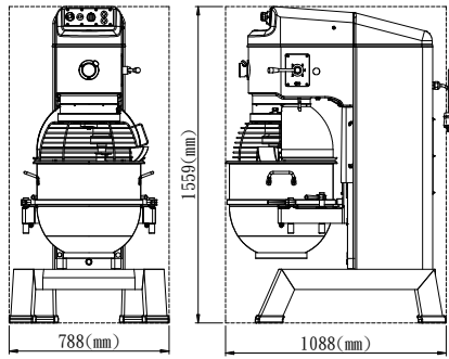
(SP-A80HI/SP-B80HI) DIMENSION
